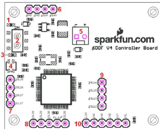
Figure 1: Controller Board
