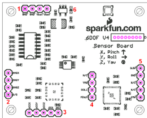
Figure 2: Sensor Board
