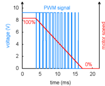
PWM speed control, showing gradual deceleration.
