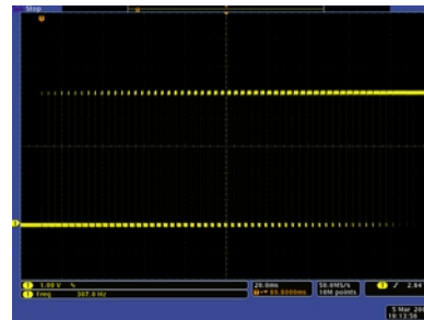
Qik 2s12v10 motor driving from speed 0 to 127 with acceleration of 28 and PWM frequency of 310 Hz.
