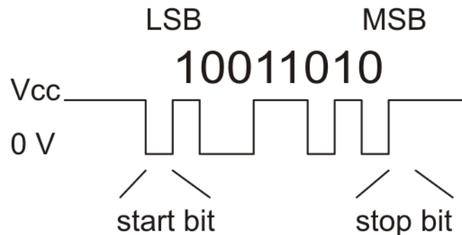
Diagram of a non-inverted TTL serial byte.
