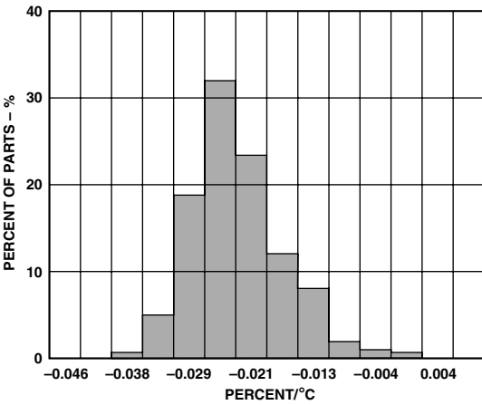
TPC 20. X-Axis Sensitivity Drift at X_{FILT} Due to Temperature Distribution, -40°C to +85°C
